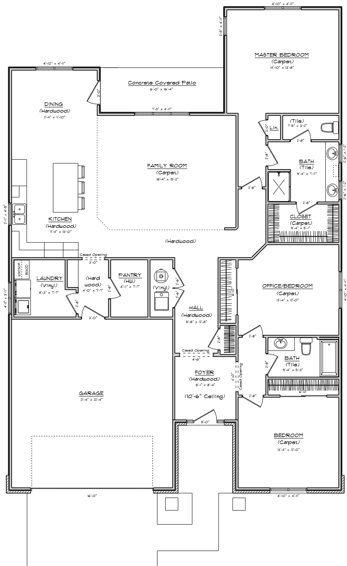
The Sedona First Floor Plan - 1910 sq. ft SCALE: 1/4" = 1'-0"
