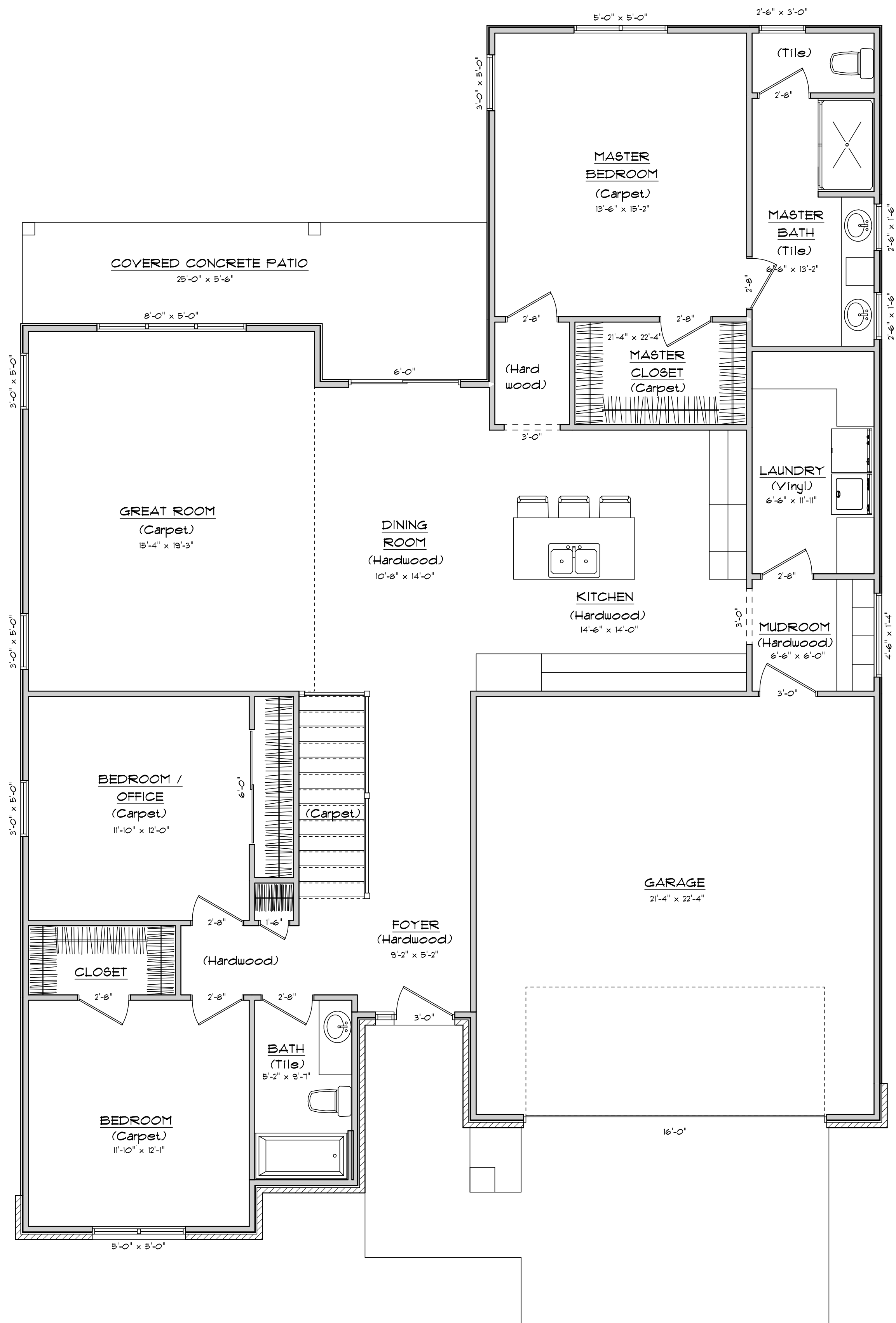
PLAN TYPE D - The Sanibel First Floor Plan on Basement 1860 sq. ft. SCALE: \frac{1}{4}'' = 1'-0''
