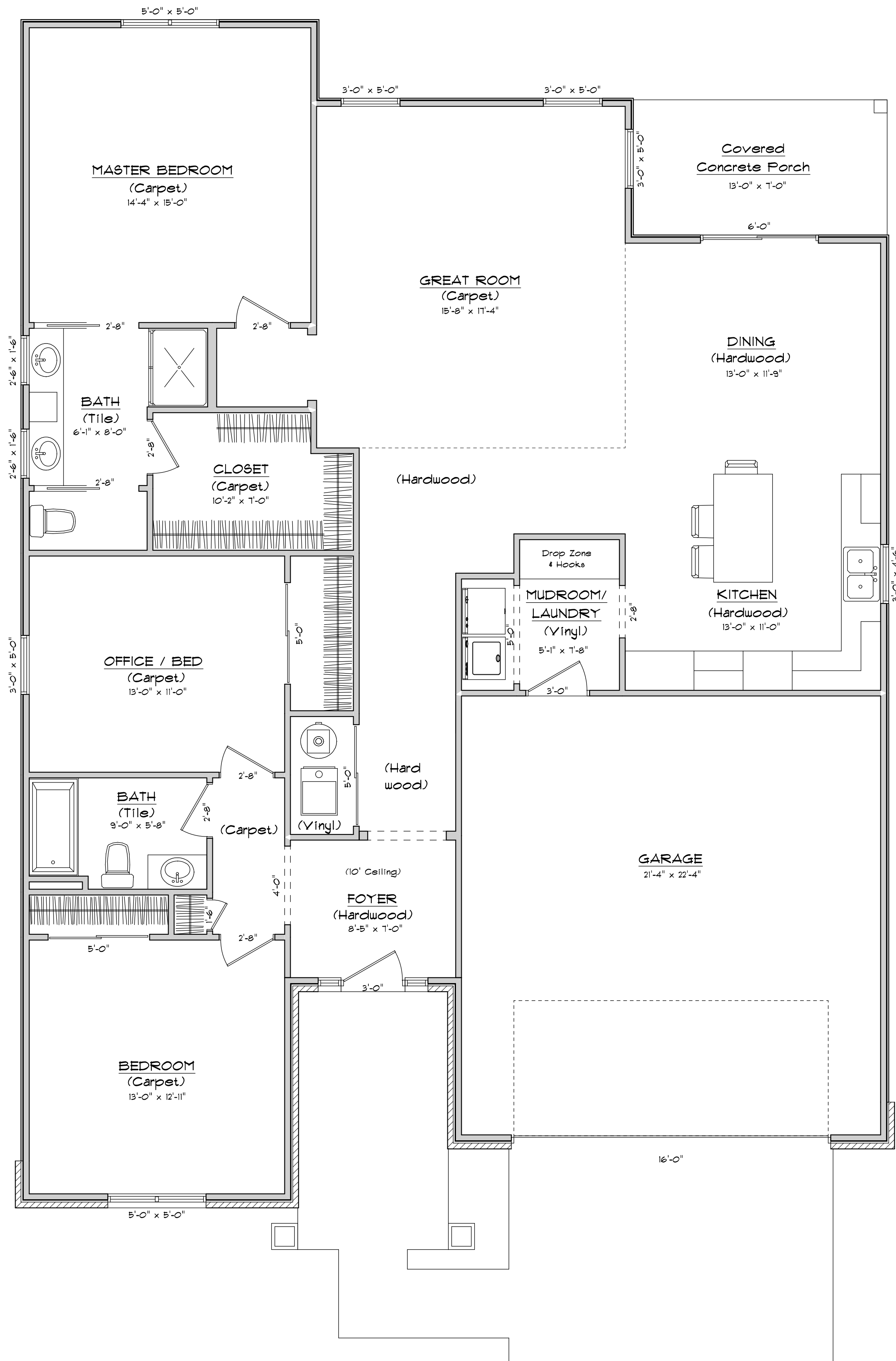
PLAN TYPE C - The Mackinaw First Floor Plan on Crawl Space - 1810 sq. ft.
